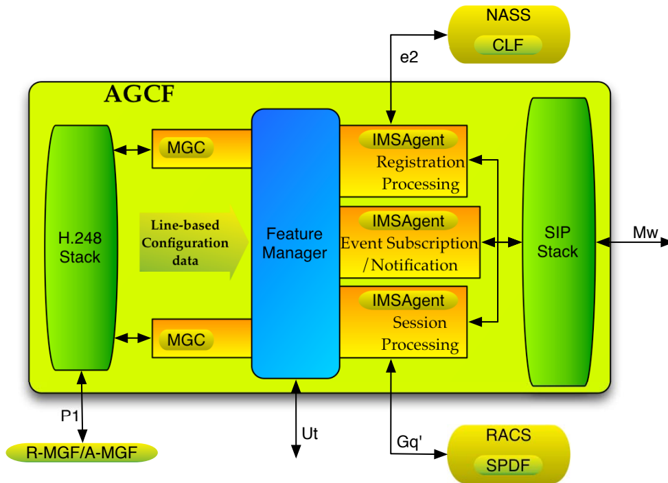
Fig 12 : AGCF functional components and interfaces
